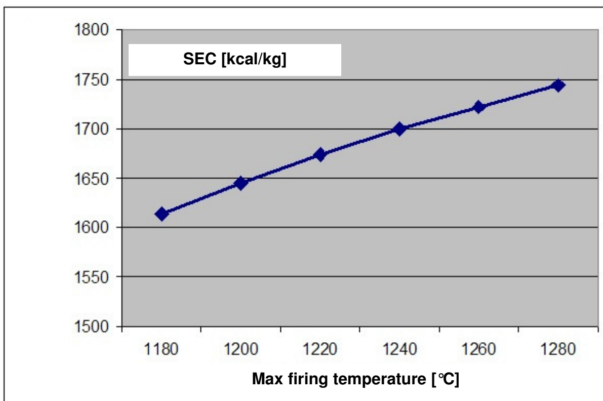
Figure 10: SEC vs. firing temperature for sanitary ware. [Friedherz Becker, Riedhammer GmbH 2007]
