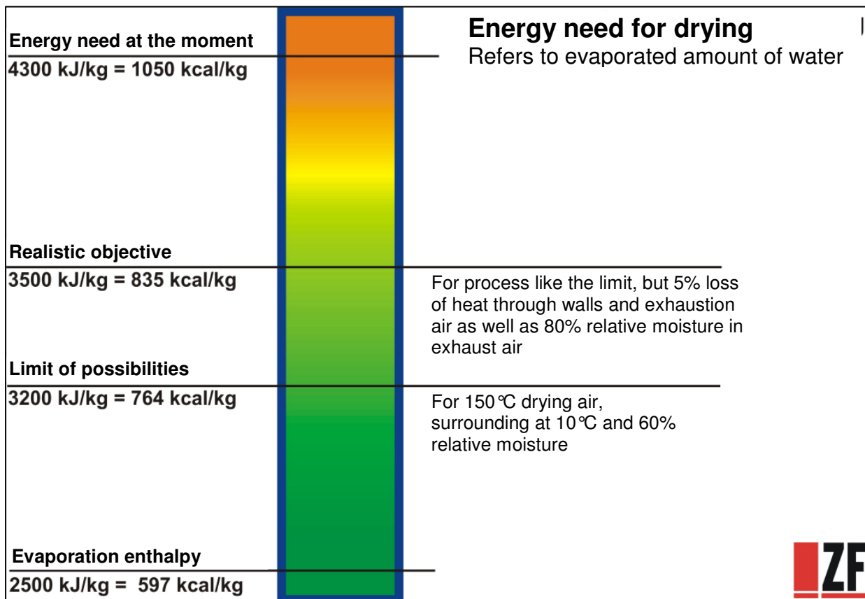
Figure 1: State of the art of drying
