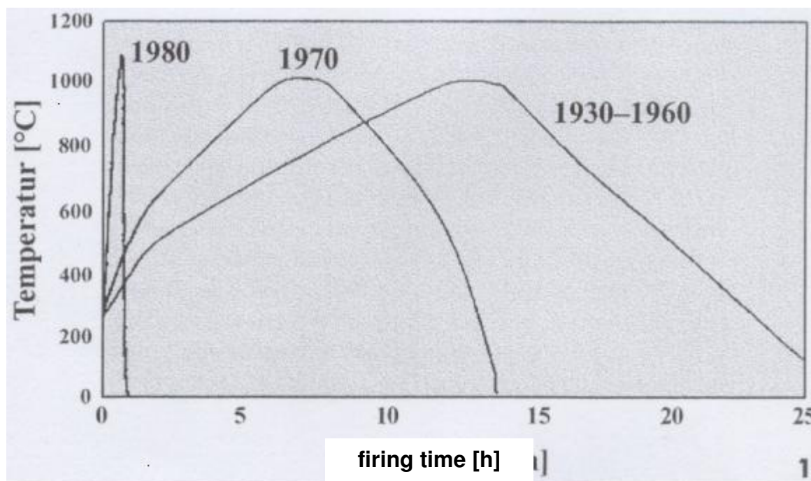
Figure 15: Decreasing firing time for tiles during the 20 th century 55
