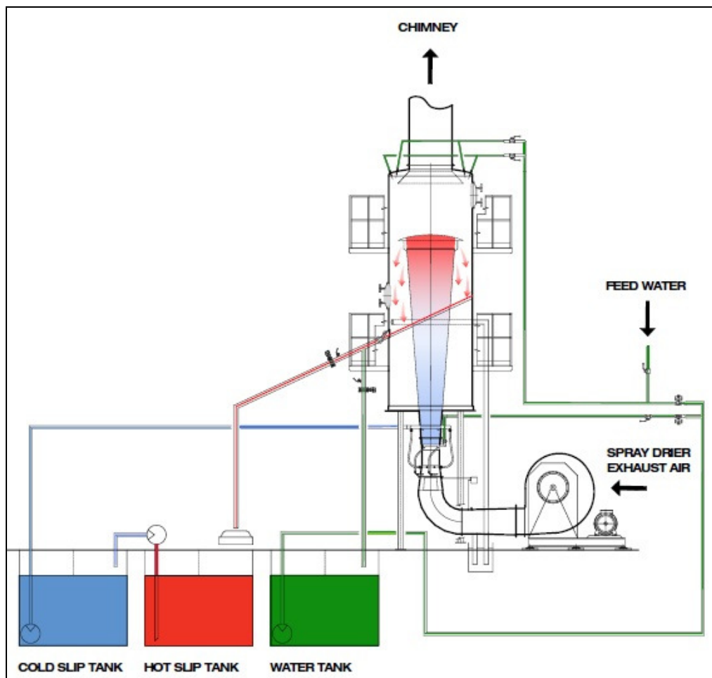
Figure 14: Dust separator for waste air from spray dryer and slip heating (by SACMI) 73
