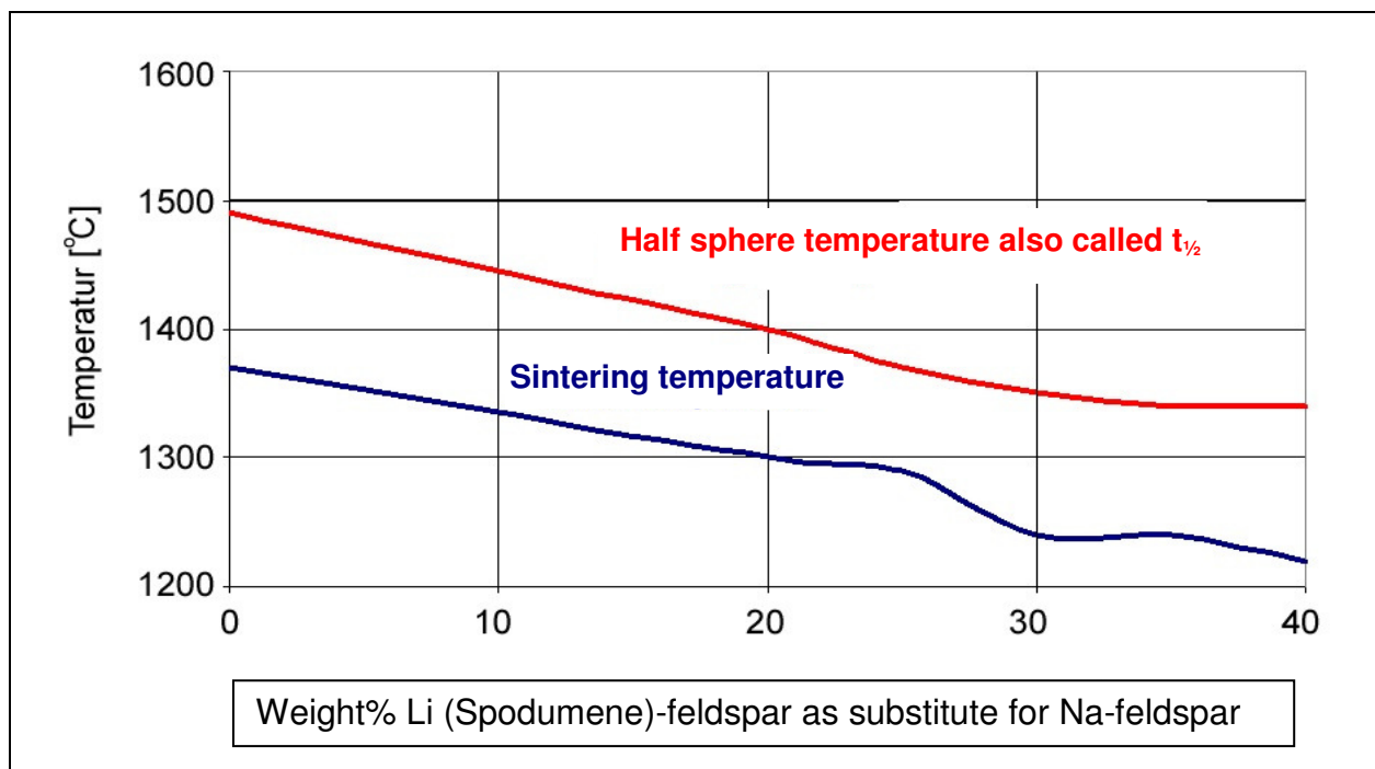
Figure 9: Effect of Li-Feldspar as sintering additive. Thierry SiliCer 2003
