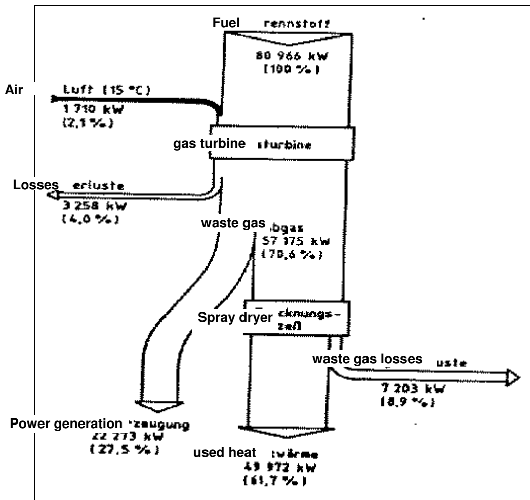
Figure 12: Balance of cogeneration of heat and power, if a spray dryer is used 56
