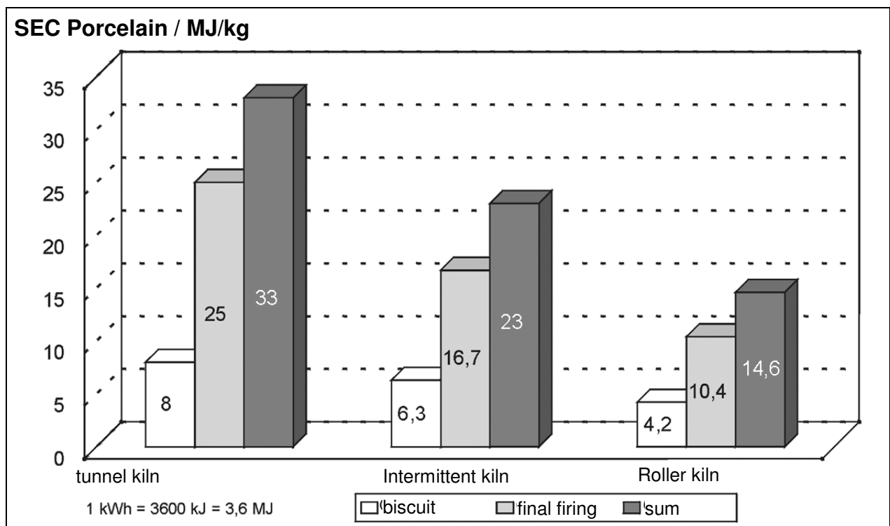
Figure 11: Comparison of different kilns for different steps of firing in table ware production
