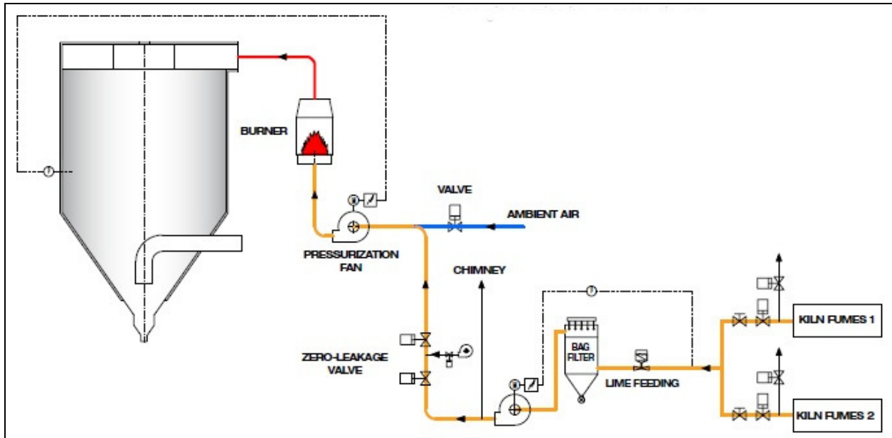
Figure 13: Recovery of cooling or fuming heat from kiln for spray drying (by SACMI) 73
